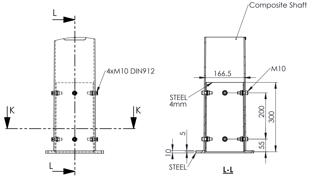
STEEL BASE SUPPORT
